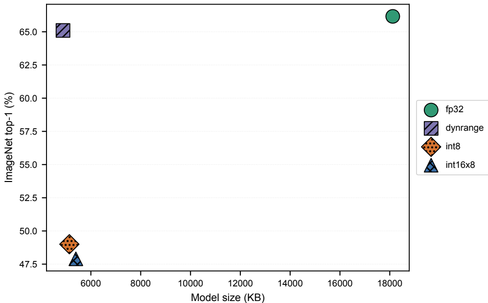
11.2.1 — TFLite size × accuracy (EfficientNet-Lite0)
