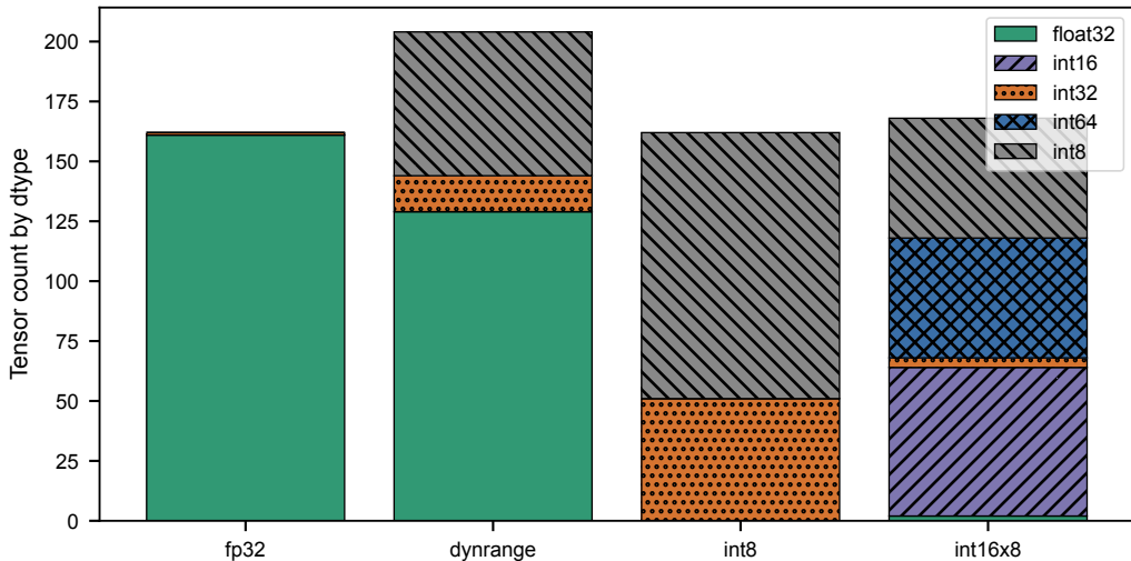
11.2.2 — TFLite per-tensor dtype map (EfficientNet-Lite0)
