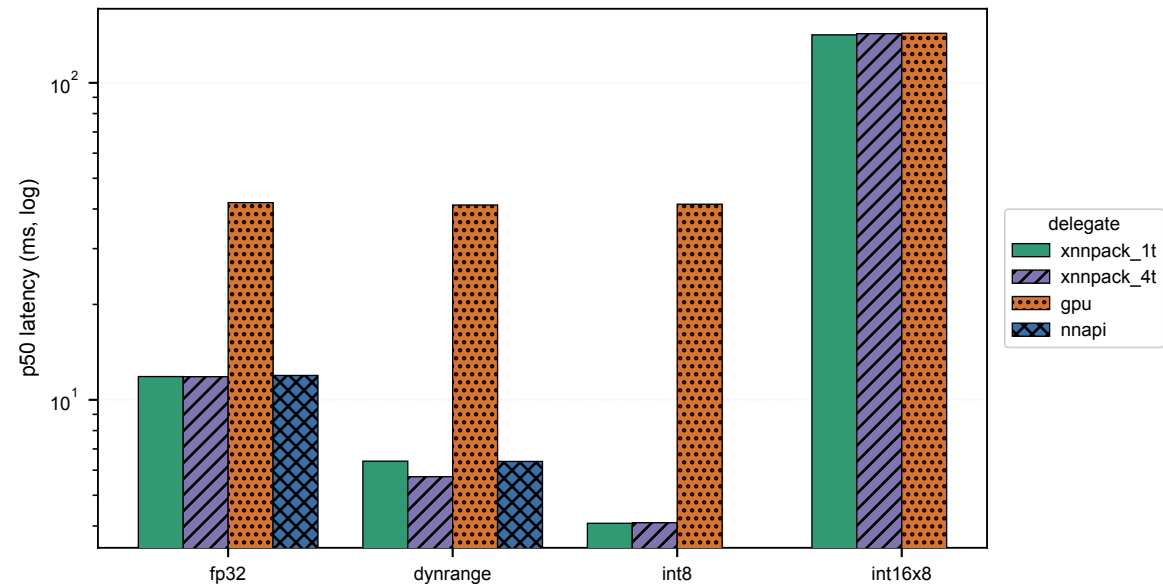
11.2.3 — TFLite p50 latency by delegate on Google Pixel 10 Pro
