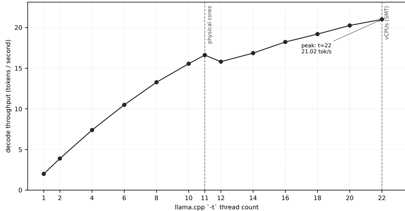
Figure 10.12 Decode throughput vs thread count, Q4_K_M Llama-2-7B
