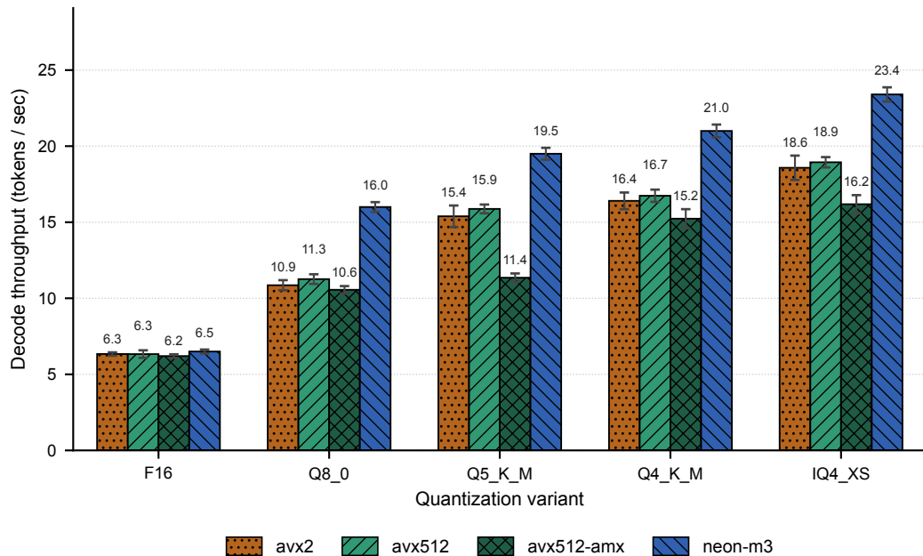
Decode throughput per kernel family on Llama-2-7B
