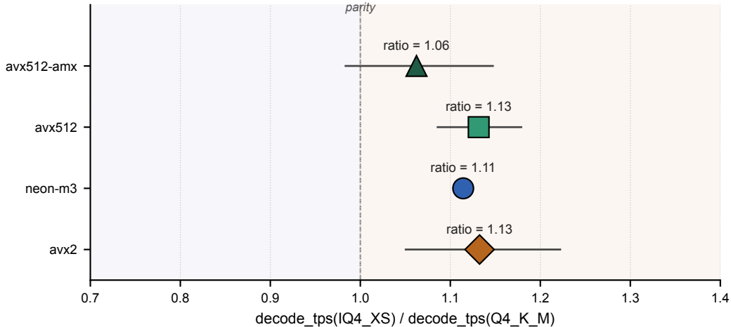
IQ4_XS / Q4_K_M decode throughput ratio per kernel family
