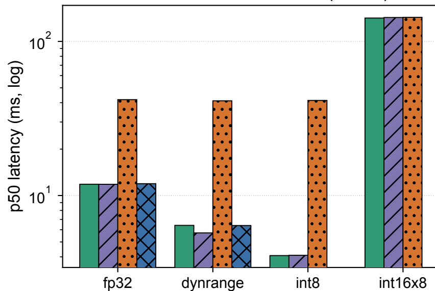
Vision — EfficientNet-Lite0 (TFLite)
