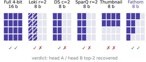
Figure 4: Bit-cells read per token by each method on the worked example (columns: channels, rows: planes). Checks mark heads ranked correctly.
