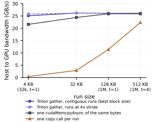
Figure 10: PCIe transfer bandwidth versus run size on the A100 host: the Triton gather of contiguous runs, a single memcpy of the same bytes, and per-run copy calls.
