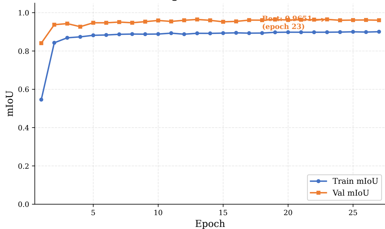
Training vs Validation mIoU
