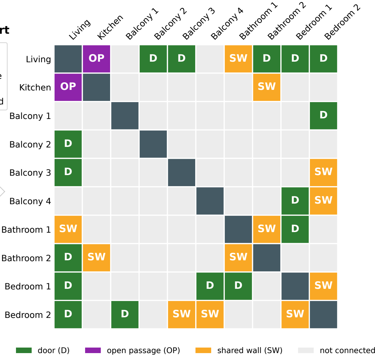
(b) Adjacency matrix
