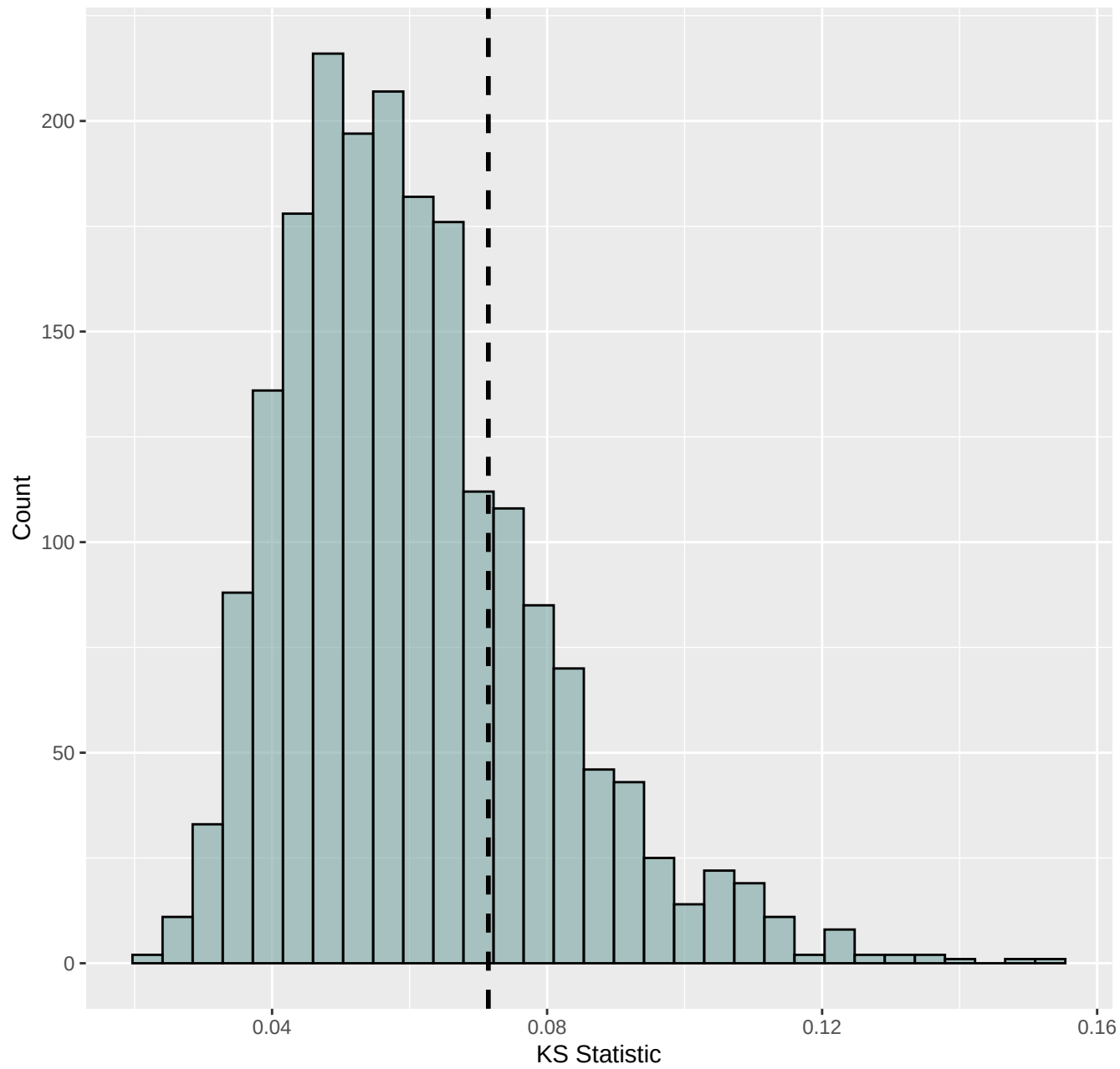
Bootstrap Distribution of KS Statistic
