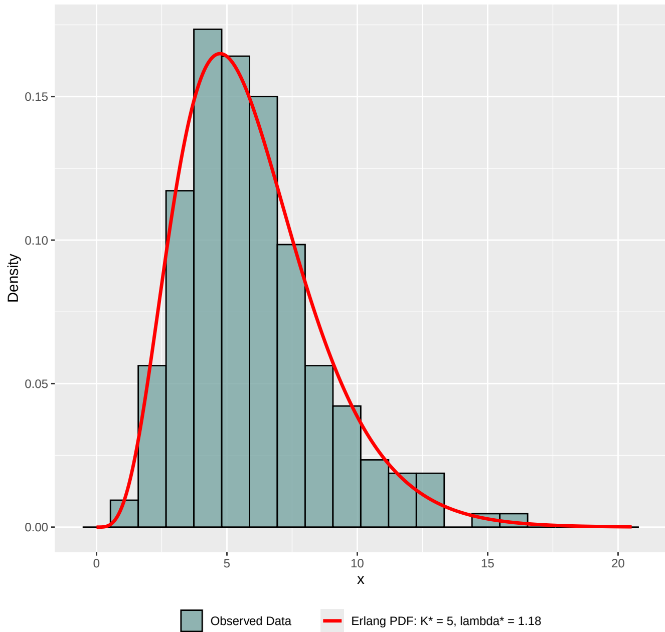
Histogram with Erlang Fits
