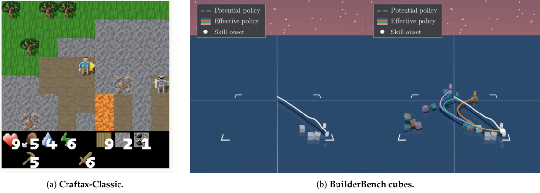
Figure 2: Empowerment maximization in large discrete and continuous environments. (a) Potential empowerment policy in Craftax-Classic [13]. The policy learns to gather resources, craft tools, then use tools to collect more resources. (b) Potential and effective empowerment policies in BuilderBench [33] with cubes in the corner. (Left) The potential policy navigates the gripper behind the cubes and stays there, preparing to control the cubes. (Right) The effective policies knock the cubes in different directions.
