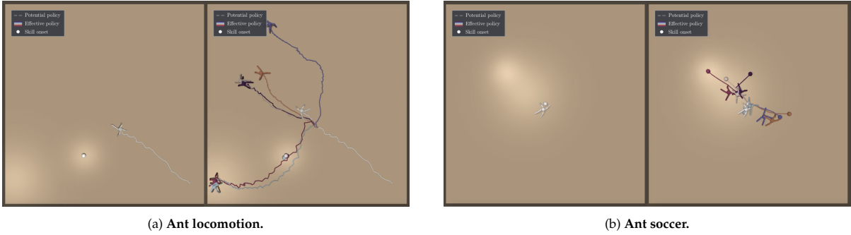
Figure 3: Empowerment maximization on high-DoF Ant tasks [34]. (a) Ant locomotion: skills cover diverse movement directions, and the potential policy navigates to states with max directional diversity. (b) Ant soccer: skills kick ball in different directions, and the potential policy positions the agent to kick and dribble the ball.
