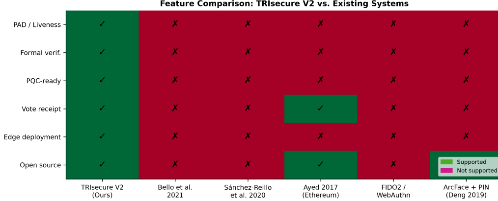
Figure 6: Feature comparison heatmap. TRIsecure V2 (left column) is the only system supporting all six binary capability flags simultaneously.
