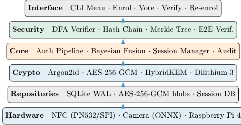
Fig. 2 TRIsSecure V2 six-layer clean architecture. Arrows indicate upward dependency direction.
