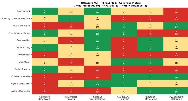
Fig. 4: Threat model coverage matrix. Green (✓, score 2) = full mitigation; yellow (∼, score 1) = partial; red (×, score 0) = no mitigation by that layer. Column sums show total defence contribution.
