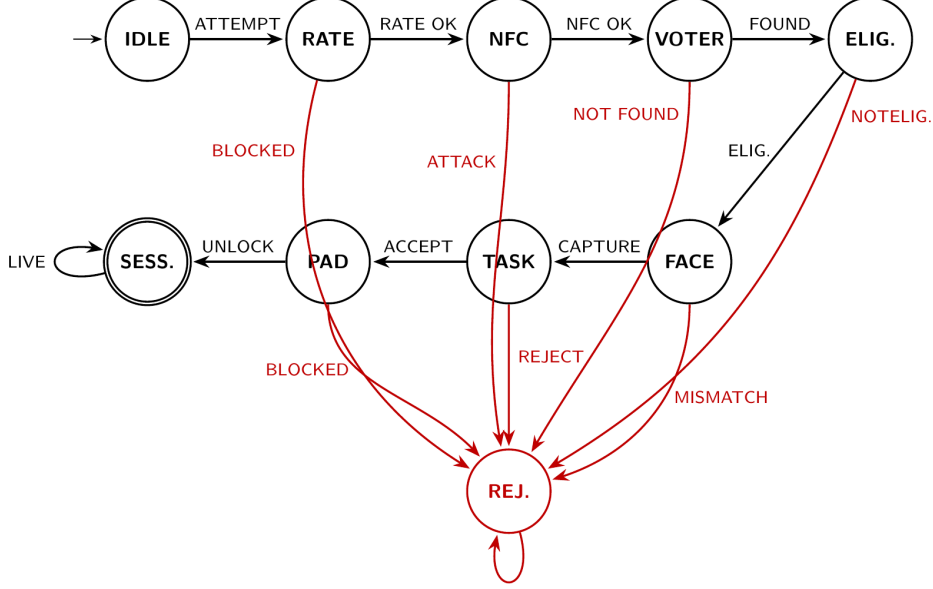
Fig. 3 TRIsure V2 authentication DFA \mathcal{M} . Black arrows show the unique canonical success path ( \text{IDLE} \rightarrow \dots \rightarrow \text{SESS.} ); red arrows denote failure transitions to the REJECTED trap state. Double circle = accepting state (SESS.).
