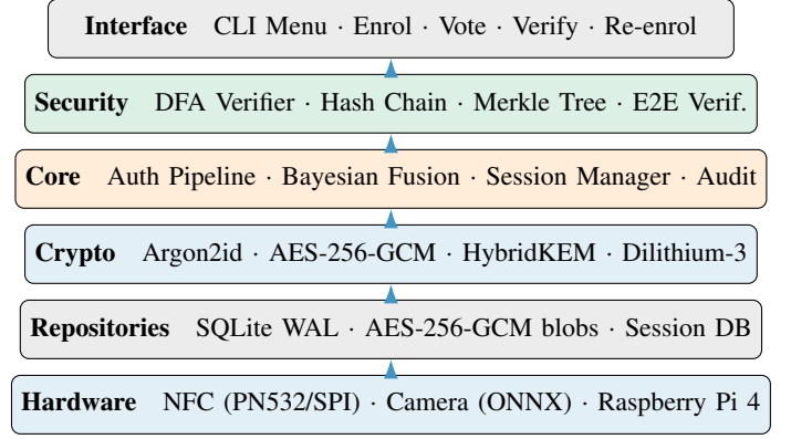
Fig. 1: TRIsecure V2 six-layer clean architecture. Arrows indicate upward dependency direction.
