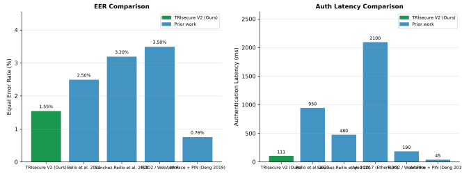
Fig. 7: EER (left) and authentication latency (right) across systems. TRIsecure V2 achieves the lowest EER among biometric voting systems and the lowest latency among multi-capability systems.
