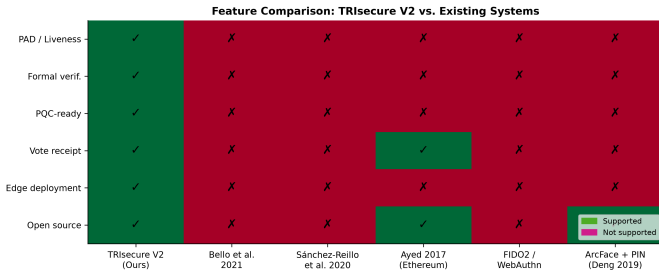
Fig. 6: Feature comparison heatmap. TRIsecure V2 is the only system supporting all six binary capability flags simultaneously.
