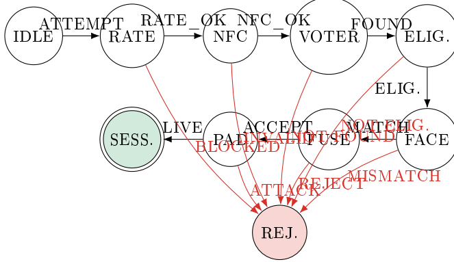
Fig. 3: TRIsecure V2 authentication DFA. Double-circle = accepting state (SESSION). Any failure transitions to REJECTED (trap state). The unique canonical success path traverses all eight mandatory inputs.
