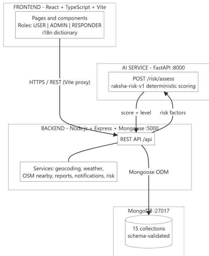
Figure 4.1: RakshaSafe System Architecture
