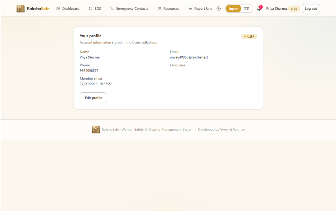
Flowchart 4.2.11: Profile
