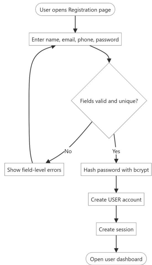
Flowchart 4.2.2: Registration
