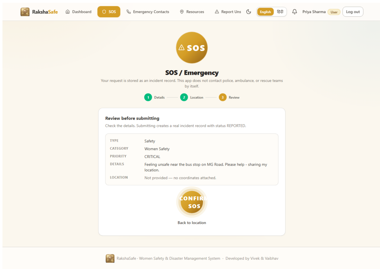
Figure B.4 - SOS step 3, review before submitting.
