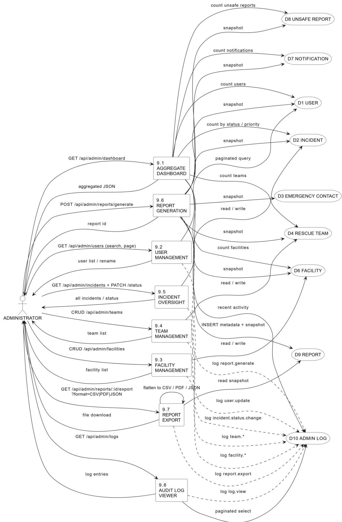
Figure 5: DFD Level 2 - Admin Dashboard & Reports
