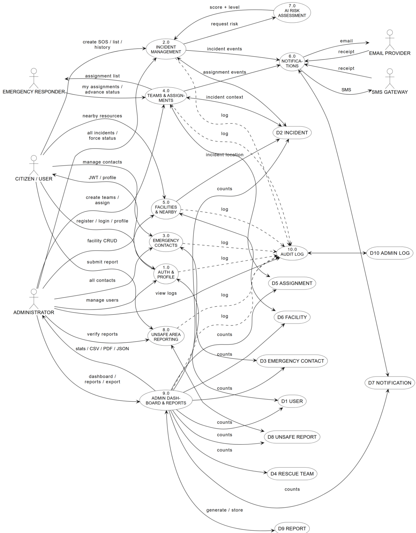
Figure 3: DFD Level 1 - Major Processes (1.0 to 10.0)
