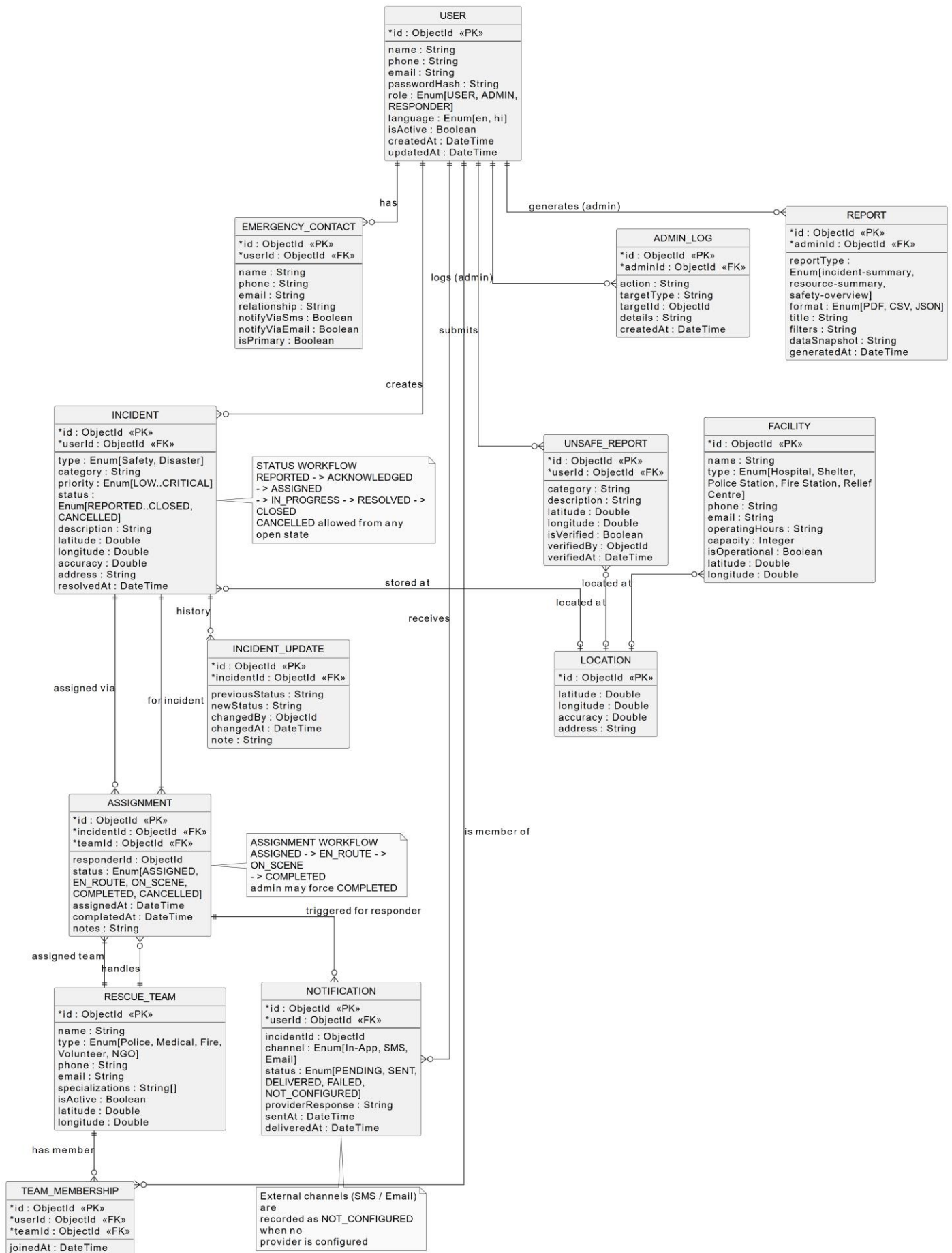
Figure 1: ER Diagram - Entity Relationship Model
