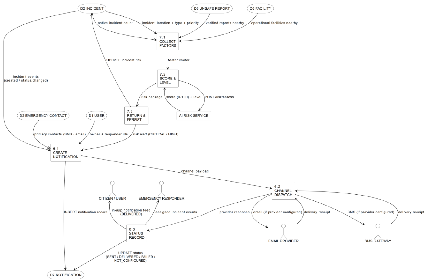
Figure 6: DFD Level 2 - Notifications & AI Risk
