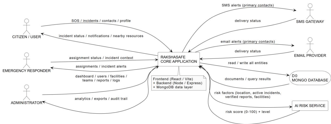
Figure 2: DFD Level 0 - Context Diagram
