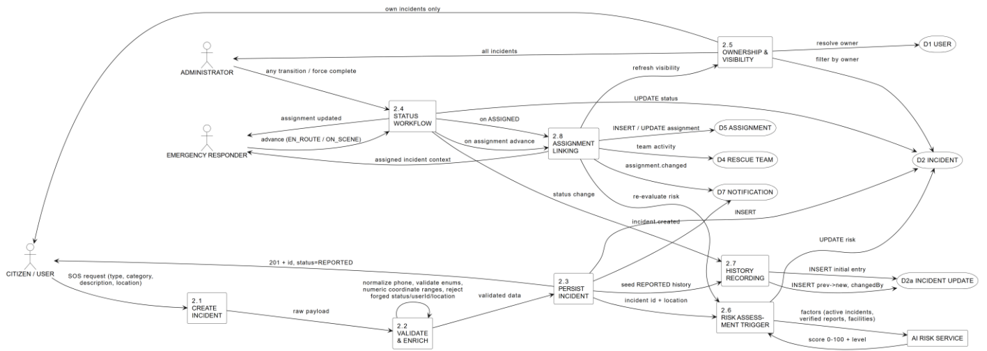
Figure 4: DFD Level 2 - Incident Management
