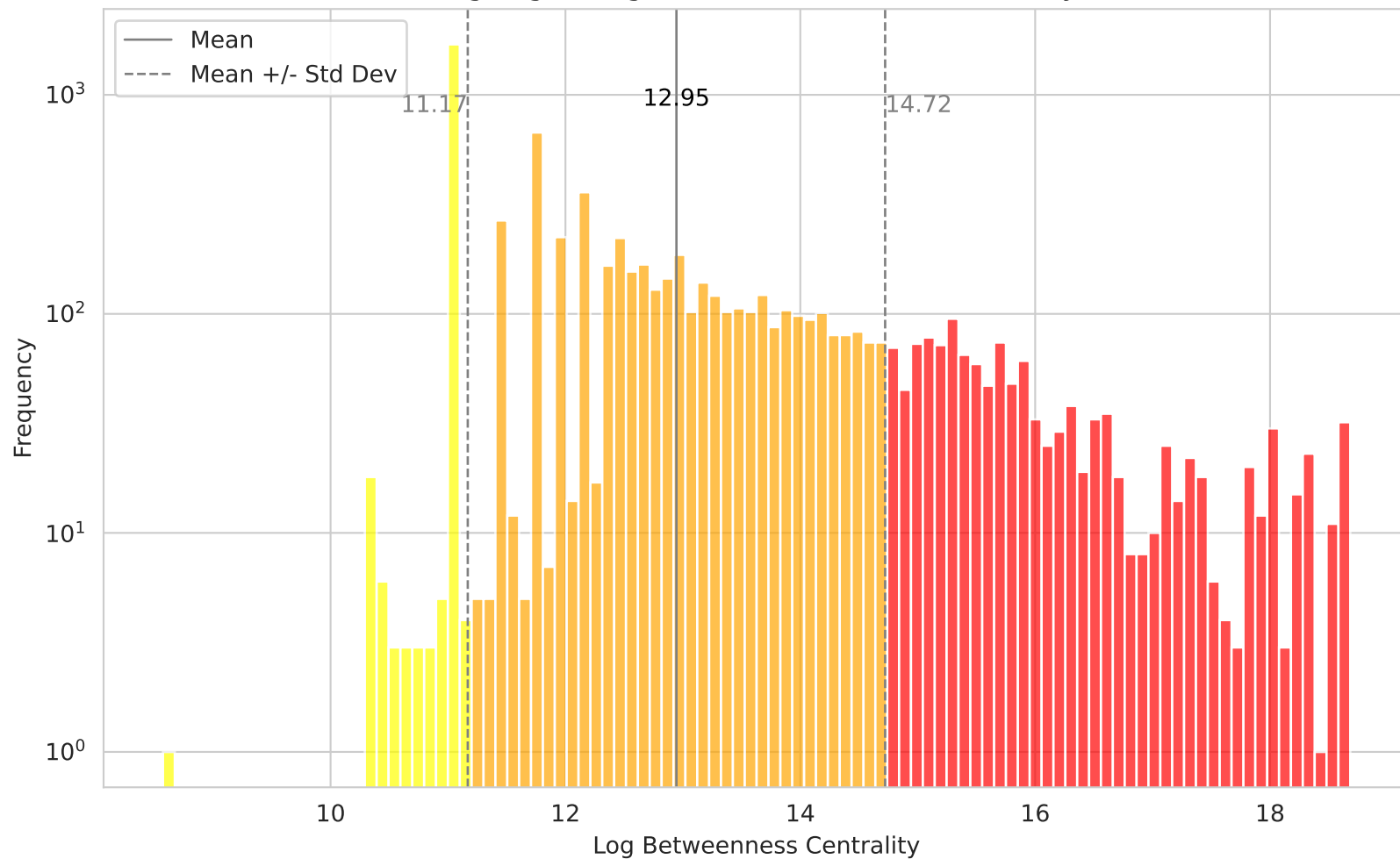
Log-Log Histogram of Betweenness Centrality
