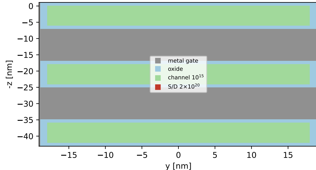
cut B-B (gate center): gate-all-around
