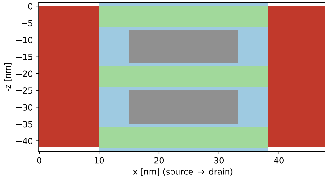
cut A-A ( y=0 ): 3-stacked nanosheets
