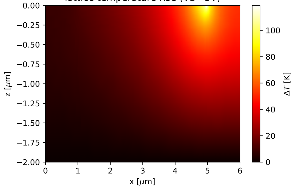
lattice temperature rise (VD=3V)
