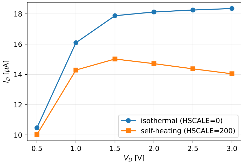
I_D - V_D droop (VG=3V, monolithic)
