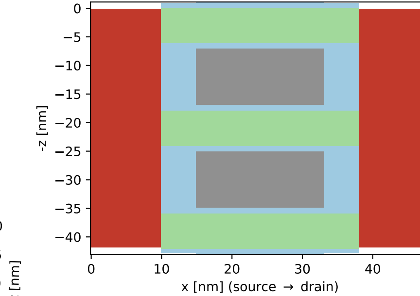
cut A-A ( y=0 ): 3-stacked nanosheets
