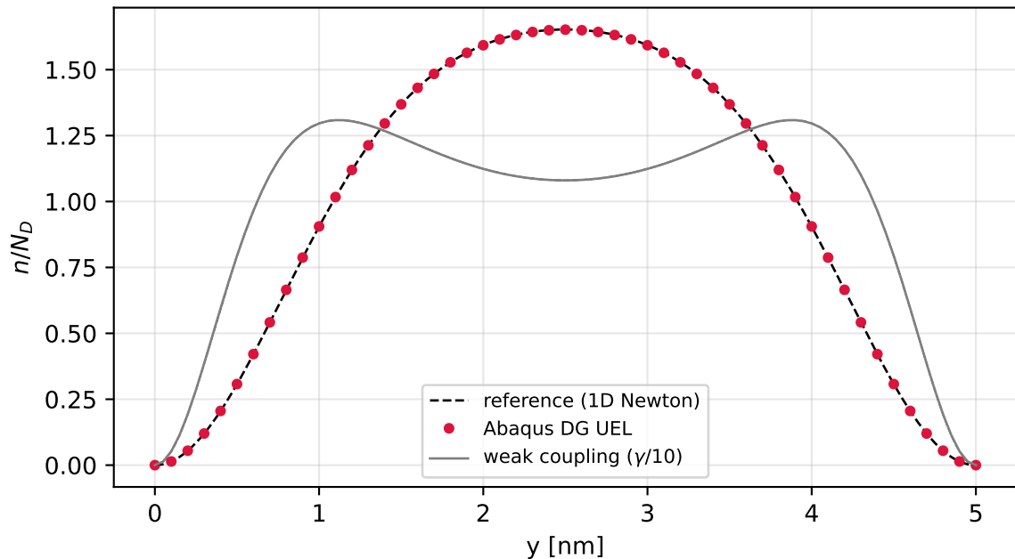
Density-gradient quantum confinement (5 nm slab, 8 \times 10^{19} \text{ cm}^{-3} )
