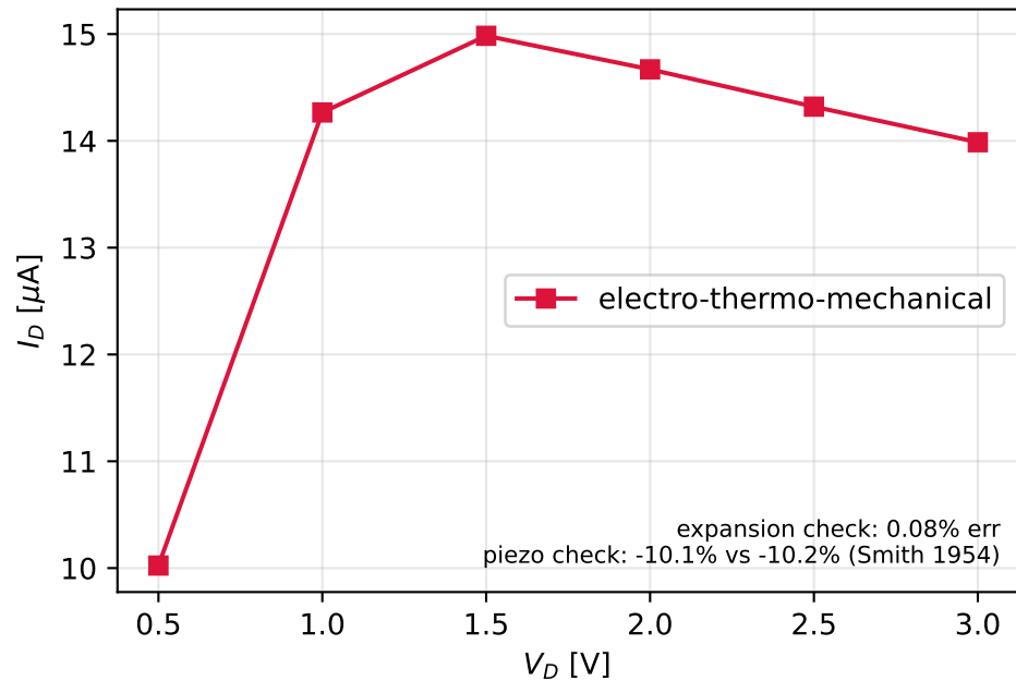
I_D - V_D ( V_G=3V , 7-dof monolithic)
