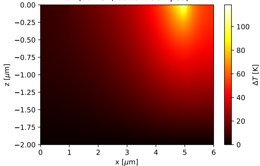
\Delta T ( V_D=3V , bottom clamped)
