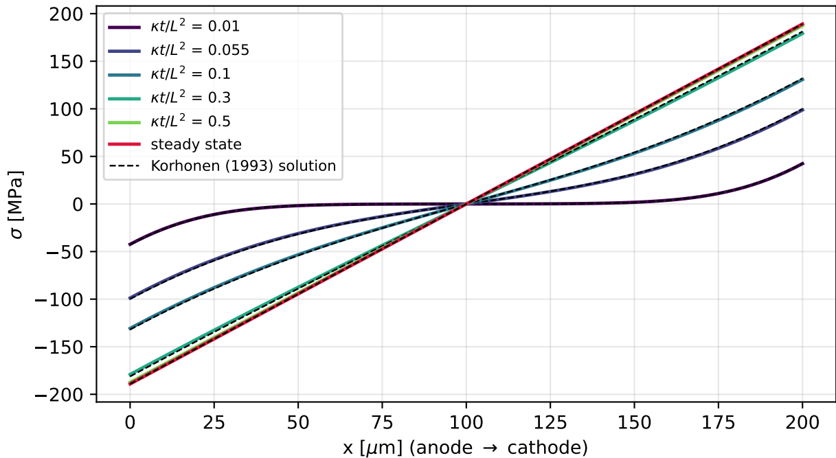
EM stress evolution: UEL vs Korhonen (1993)
