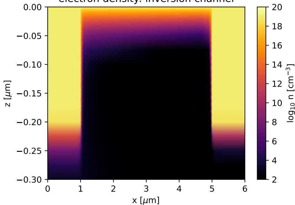
electron density: inversion channel
