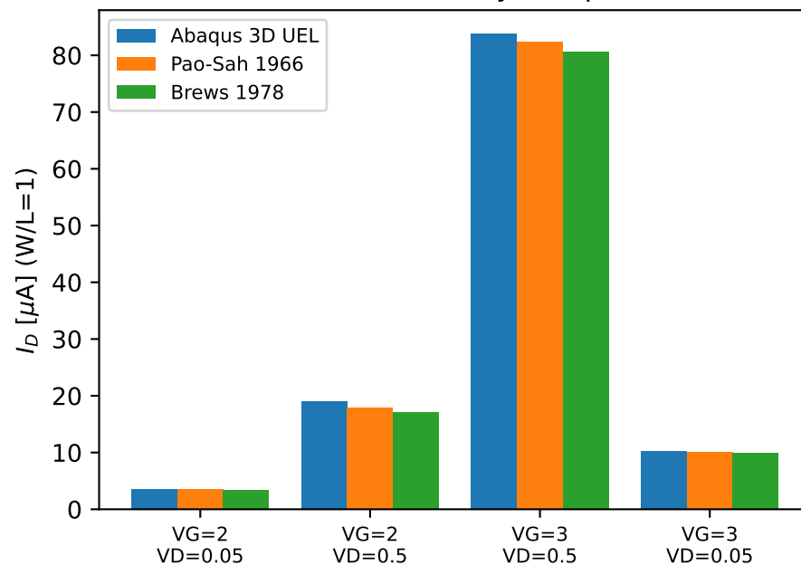
drain current: 3-way comparison
