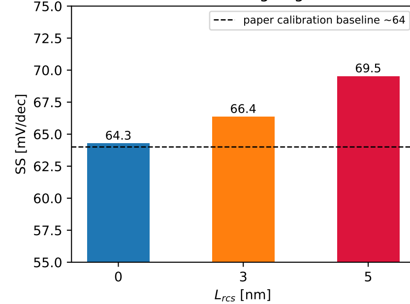
subthreshold swing degradation
