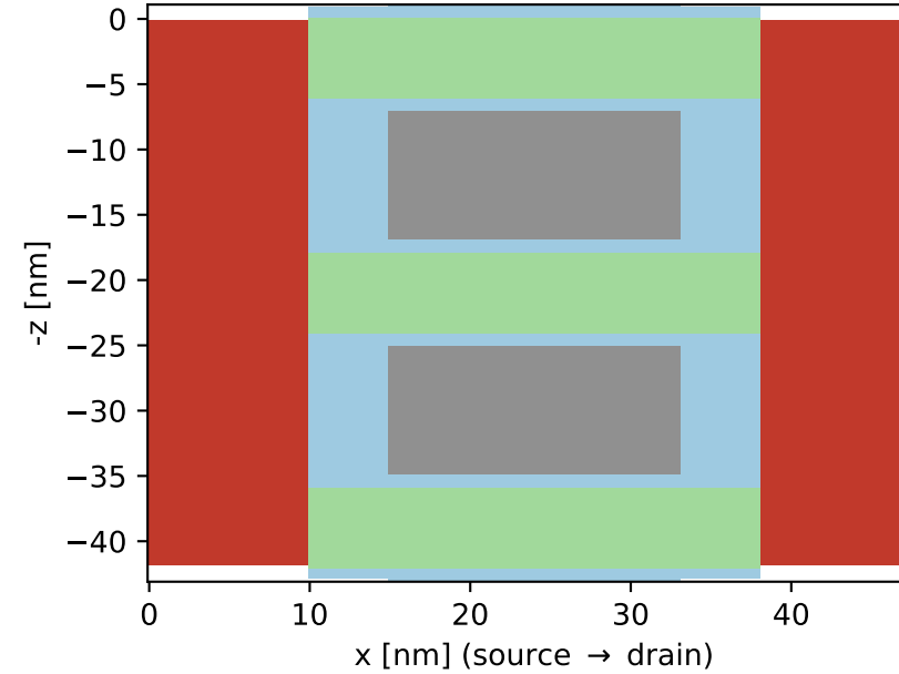
cut A-A ( y=0 ): 3-stacked nanosheets
