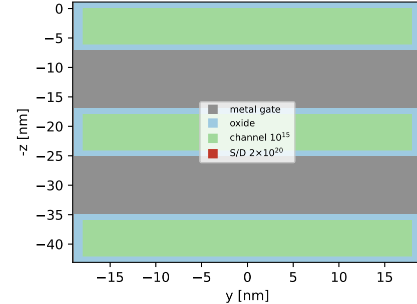
cut B-B (gate center): gate-all-around
