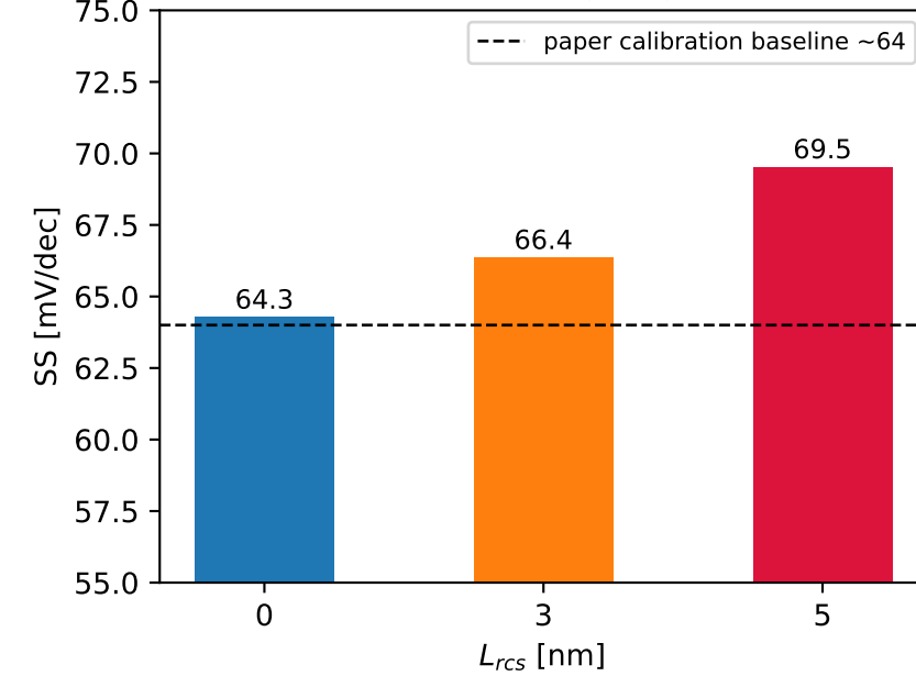
subthreshold swing degradation
