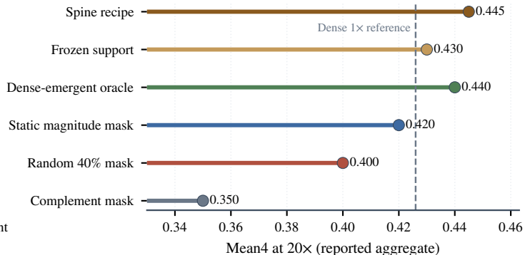
D Dynamic support beats arbitrary controls
