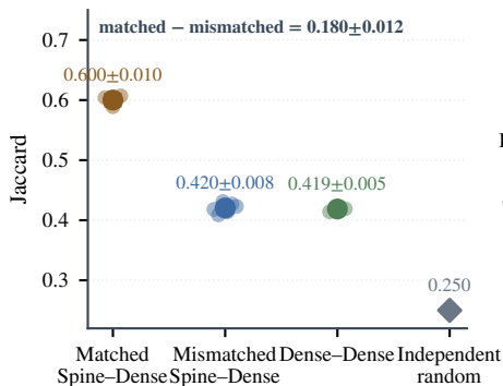
C Alignment exceeds structured nulls
