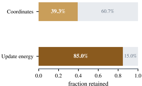
A A small support carries most update energy
