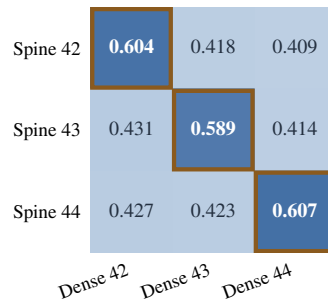
B Matched seeds form a clean diagonal
