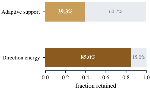
A A small support carries most direction energy
