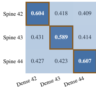
B Matched seeds form a clean diagonal
