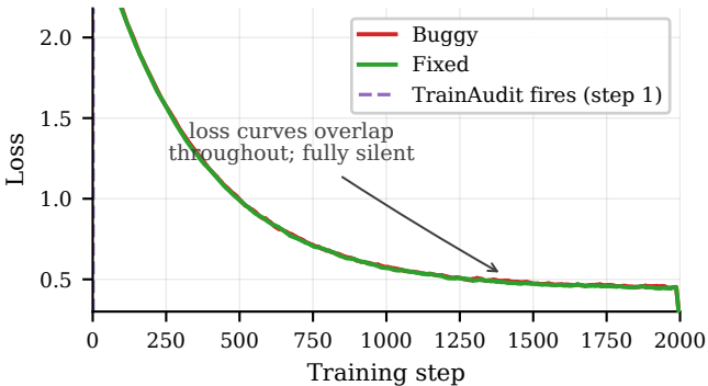
Case 1 - SFT prompt-format: training loss
