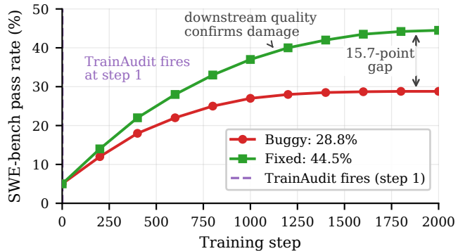
Case 1 - downstream quality diverges
