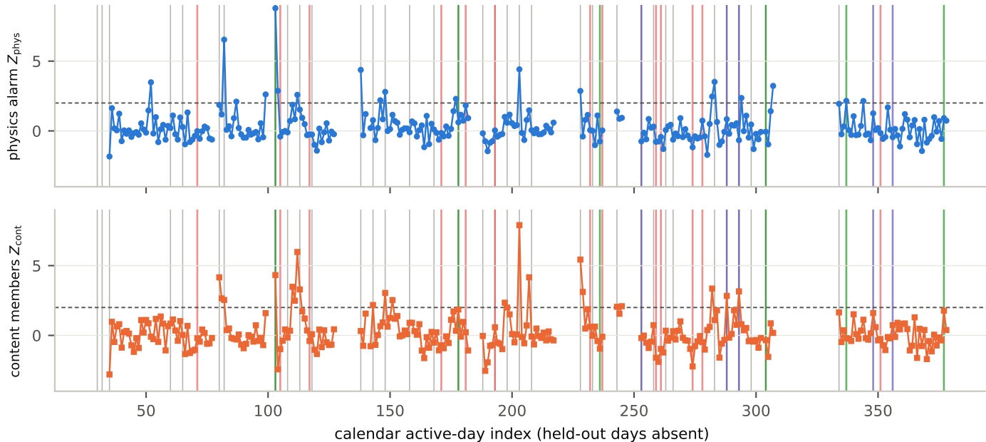
Daily alarm scores; vertical lines: goal kickoffs (gray), room (violet), scaffold (red), roster (green)
