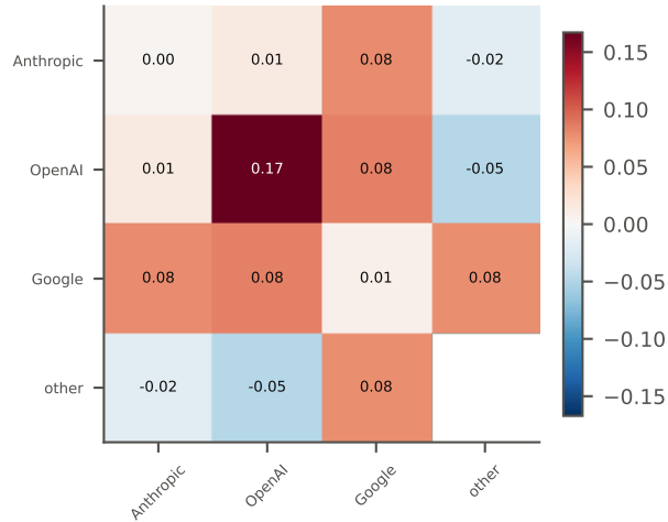
talk spins: K \times K mean-field J ; \Delta = 0.029 ( p = 0.24 )
