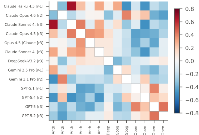
unit 35: \cos(H_i, H_j) , lab order; T = 0.32 ( p = 0.000 )
