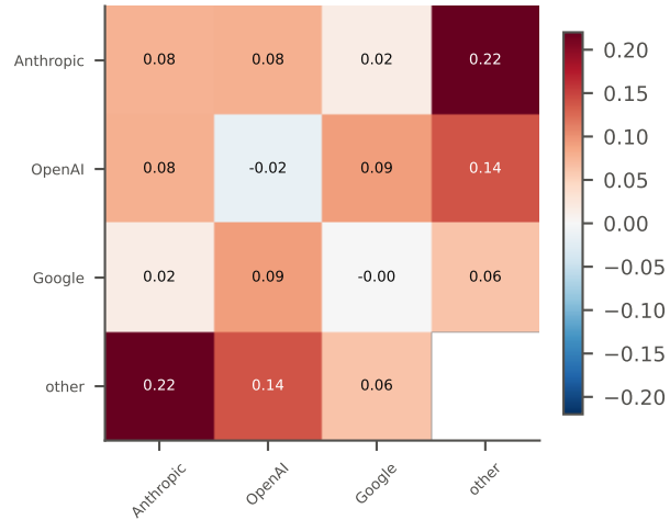
content co-movement: K \times K mean-field J ; \Delta = -0.028 ( p = 0.49 )
