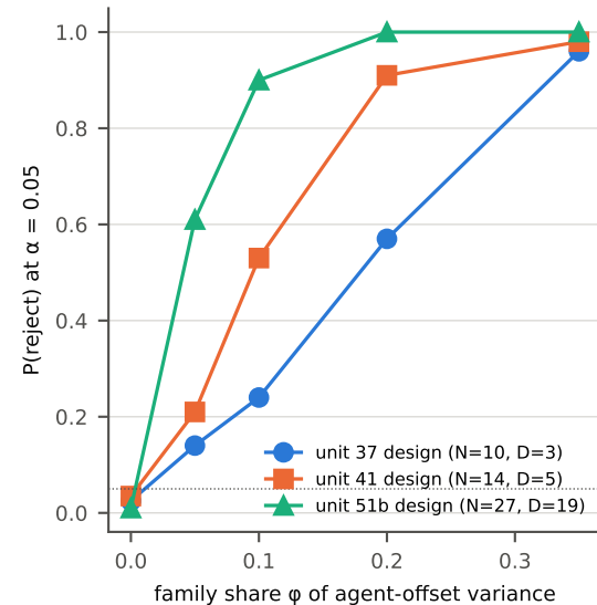
F1 family-field test: size and power
