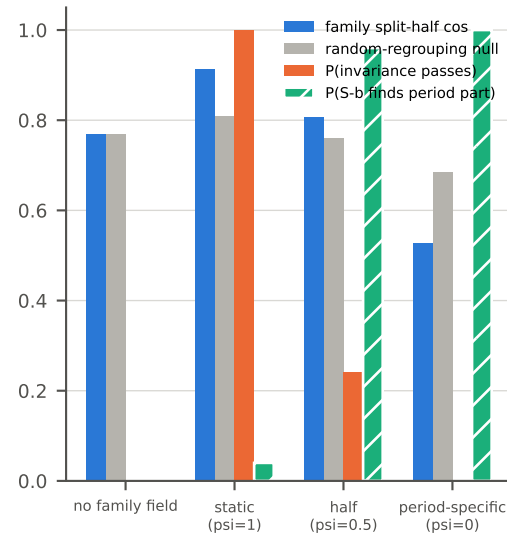
F2 invariance and fixed-offset rival
