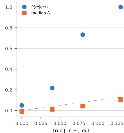
F3 content K×K (N = 14, 40 windows)
