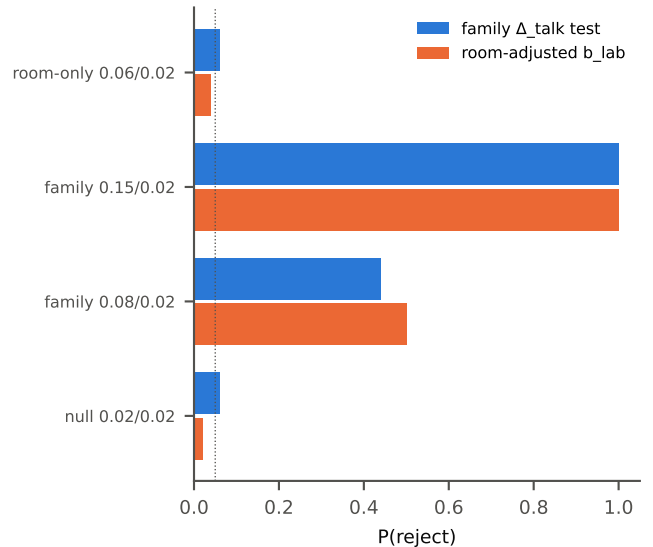
F4 talk spins (kinetic Ising, #41 design)
