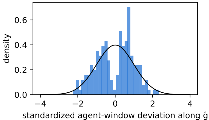
G12: shape ( \gamma = -0.38 )
