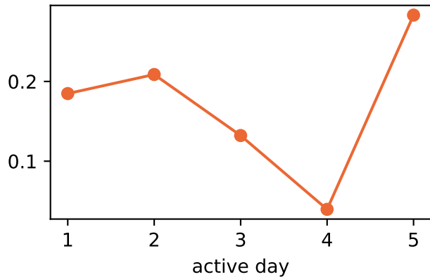
g = 0.70 [0.56, 0.75]
