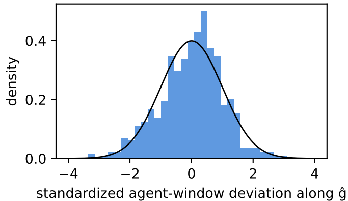
G38: shape ( \gamma = -0.60 )
