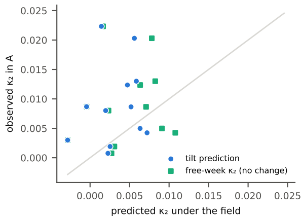
(c) P2: \rho = 1.00 [-0.42, 1.94]; transverse \rho \perp = -0.12
