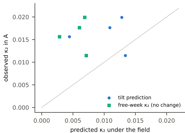
(c) P2: \rho = 0.44 [-0.18, 1.54]; transverse \rho_{\perp} = 0.28
