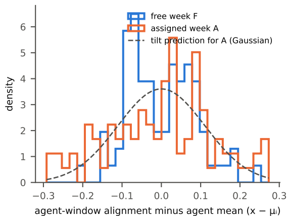
(c) P2: \rho = 0.44 [-0.18, 1.54]; transverse \rho_{\perp} = 0.28
