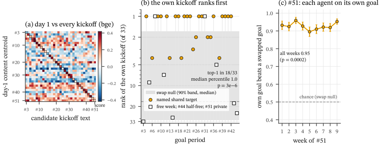
FIG. 6. Day-1 content lands on its own kickoff text. (a) Each row is one goal period’s day-1 centroid, scored against all 33 kickoffs; the diagonal is the own kickoff. (b) The own kickoff ranks first in 18 of 33 periods. The gray band is the swap null; the misses are kickoffs with no shared target. (c) In #51 each agent sits closer to its own private goal than to another agent’s goal in 0.95 of pairs, for nine weeks.
