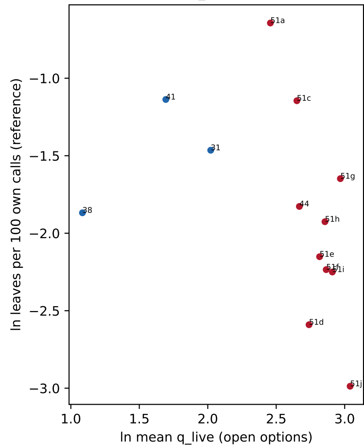
O4 across units: b_q = -0.32 [-4.52, 5.34]
