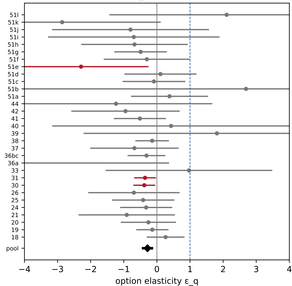
attention: \epsilon_q per unit (95% CI)
