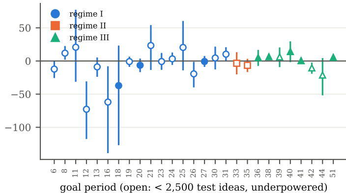
(a) held-out gain of seed features over the strongest baseline
