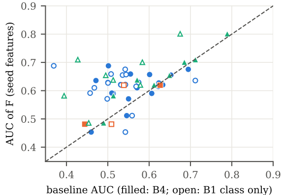
(b) held-out AUC, reach \geq 2 in 24 h
