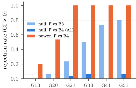
(a) synthetic size and power on real features
