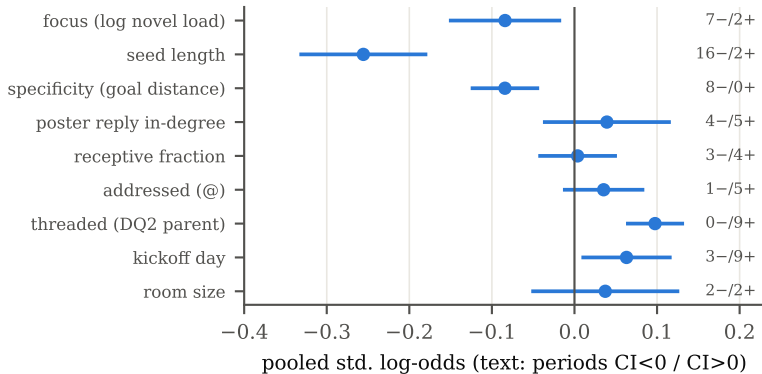
(b) which seed features carry fitness
