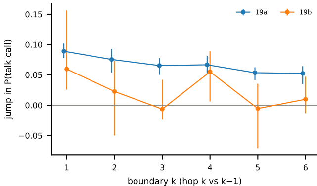
G19: peer message \rightarrow recipient
