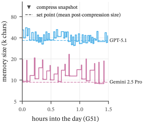
(a) sawtooth around a set point
