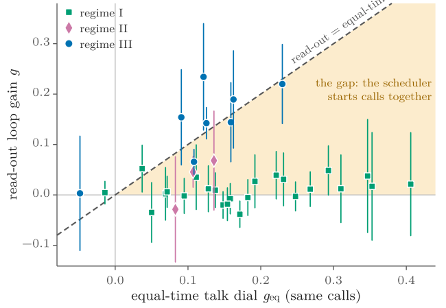
FIG. 21. The scheduler impostor, measured (H67). Each point is a goal period. The equal-time dial g_{eq} counts how much agents talk in the same calls. The read-out gain g counts only the response to a message that a call reads. In regime I (green squares) the equal-time dial is large, but the read-out gain is near zero. Agents talked together because the scaffold scheduled their calls together, not because they read each other. In regime III (blue circles) the two agree. Look at the orange gap between the green points and the diagonal: that gap is the impostor.
