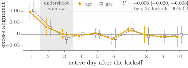
b #51: two decay rates
