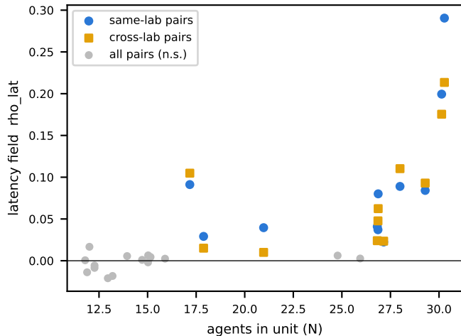
a turnaround co-moves across providers, more at large N
