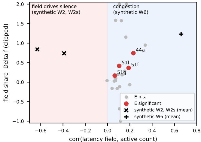
b the sign says load, not drive
